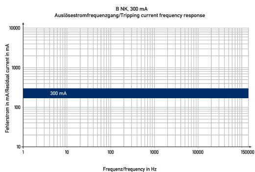
Diagramme FI-/LS-Kombinationen DRCBO 4 Bo6/0,30/3N-B NK
