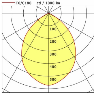
Flixx 300 Flat Round (FLIRZ 300.05, 1xLED 29W 830/3000K 2810lm 85 °)
