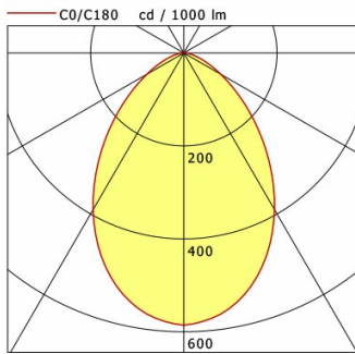
Flixx 300 Flat Round (FLIRZ 300.24, 1xLED 29W 830/3000K 2620lm 85 °)
