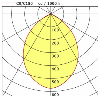
Flixx 300 Flat Round (FLIRZ 300.25, 1xLED 29W 830/3000K 2730lm 85 °)
