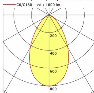
Flixx 300 Square (FLIQZ 300.24, 1xLED 26W 840/4000K 2760lm)
